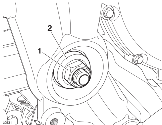
1. Lock nut 2. Adaptor
