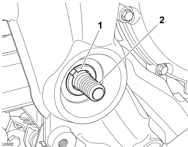
1. Right hand swinging arm adjuster 2. Swinging arm spindle
