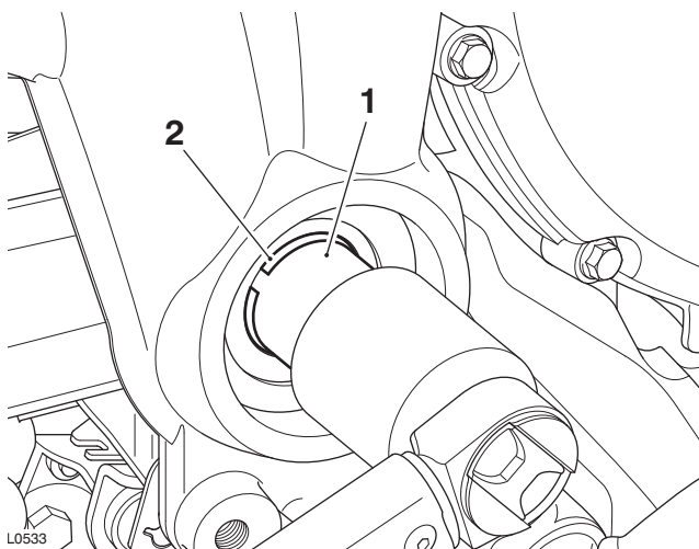
1. Service tool T3880182 2. Swinging arm frame adjuster
